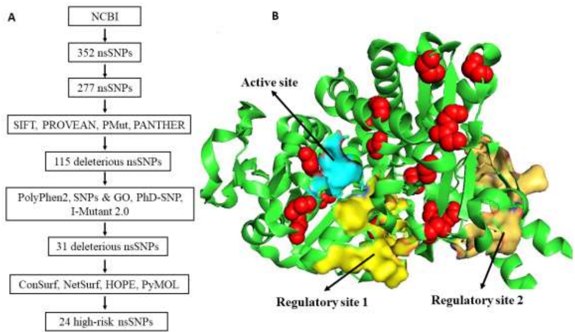
Figure 4. A) The flowchart of the steps to screen and identify the high-risk nsSNPS in NT5C2 using bioinformatics tools and B) The structure of the 5'-nucleotidase (NT5C2) enzyme illustrated by PyMOL: The active site and regulatory sites 1 and 2 are marked in blue, yellow and orange, respectively. Also, 24 high-risk mutations are demonstrated with red spheres.
