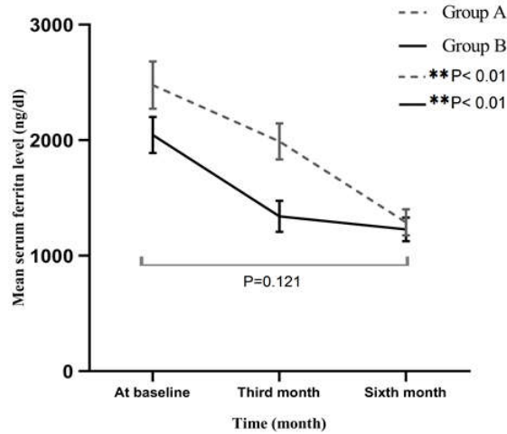
Figure 2. Line graph represent means ± SEM of serum ferritin level in A and B groups (n= 53 in group A and 54 in group B). Group A received Deferasirox and Deferiprone; group B received Deferoxamine and Deferiprone for 6 months. Serum ferritin level was evaluated on: 0, 3 and 6 months after treatment. ** P <0.01 significantly different within group A and B. P= 0.121 no significant difference in decreasing the level of serum ferritin between the two groups
