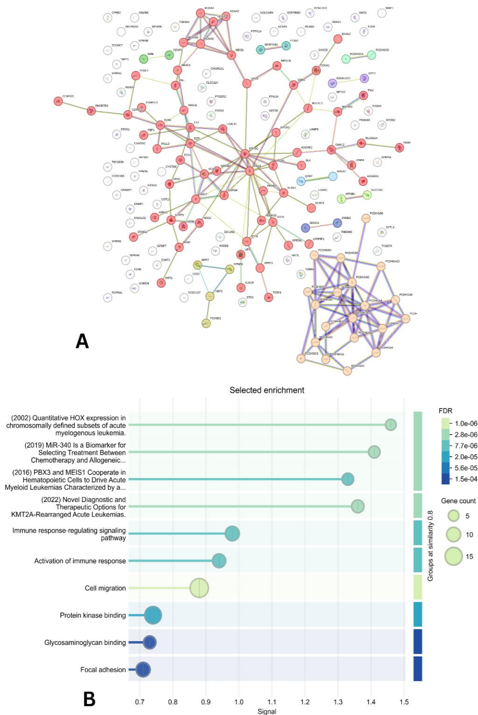
Figure 2. Shows the PPI-based clustering of upregulated DEGs (A) and the functional enrichment analysis of these upregulated genes in 11q ALL (B)
