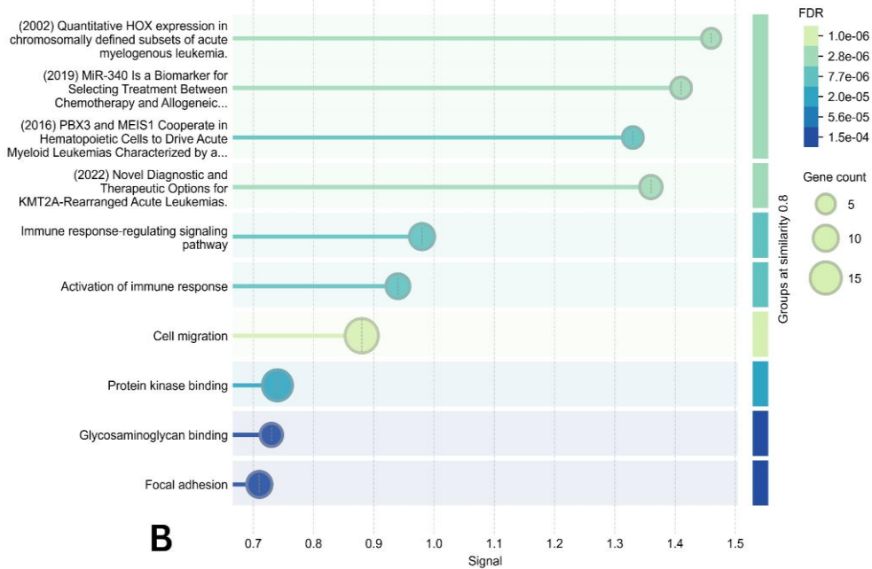
Figure 2. Shows the PPI-based clustering of upregulated DEGs (A) and the functional enrichment analysis of these upregulated genes in 11q ALL (B)
