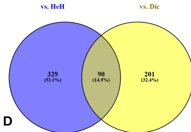
Figure 1. Illustrates the DEGs in 11q ALL compared to dic(9;20) ALL and HeH ALL individuals. Figure 1(A) shows the number of upregulated and downregulated genes in 11q ALL compared to dic(9;20) ALL. Figure 1(B) shows the number of upregulated and downregulated genes in 11q ALL compared to HeH ALL. Figure 1(C) and Figure 1(D) show the commonly upregulated and downregulated genes when 11q ALL individuals are compared to both dic(9;20) and HeH.
