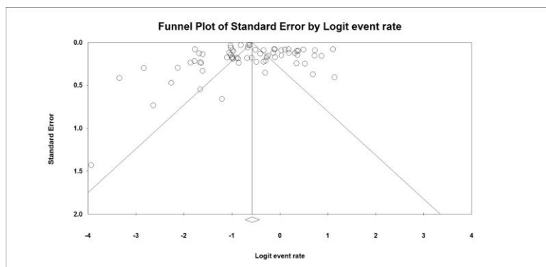
Figure 10. Funnel plot
